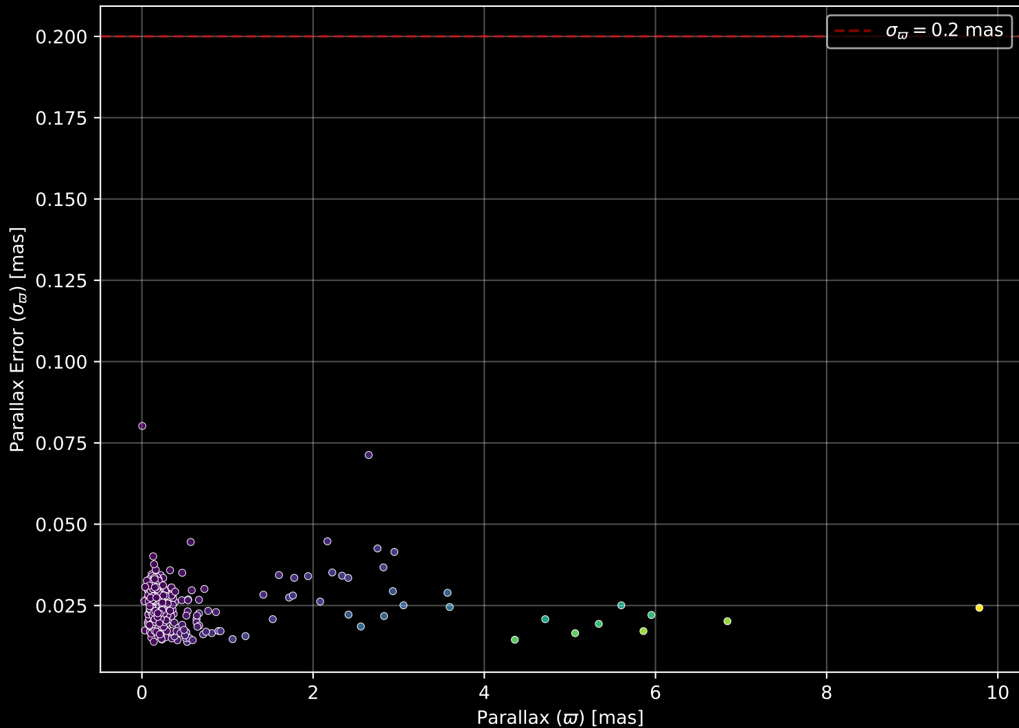
APOGEE DR17 Field: [345+14] Parallax Quality (n= 302)
