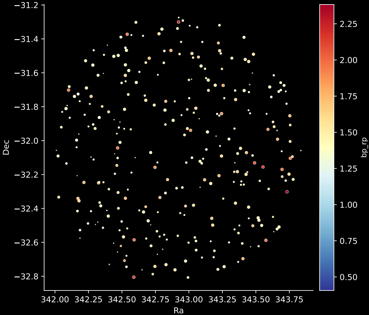
APOGEE DR17 Field: [345+14] Stars: 302
