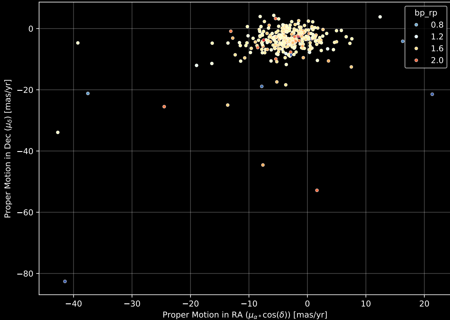
APOGEE DR17 Field: [345+14] Proper Motion Diagram (n= 302)
