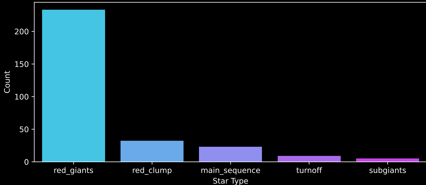
APOGEE DR17 Field: [345+14] Count plot of Star Type
