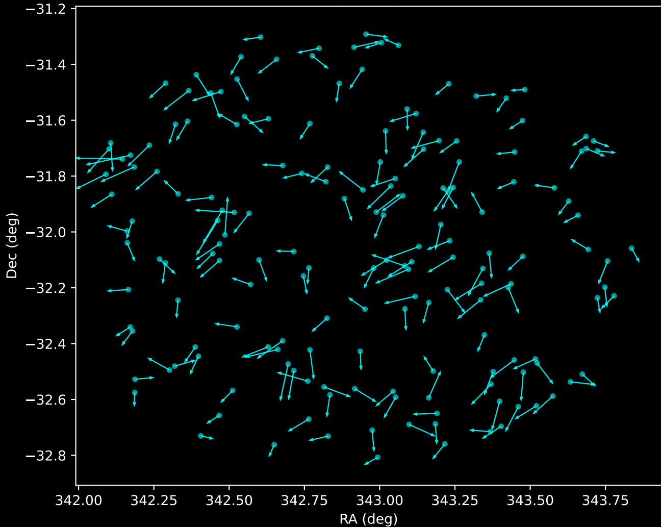
APOGEE DR17 Noise Stream Proper Motion Vectors (n=172)
