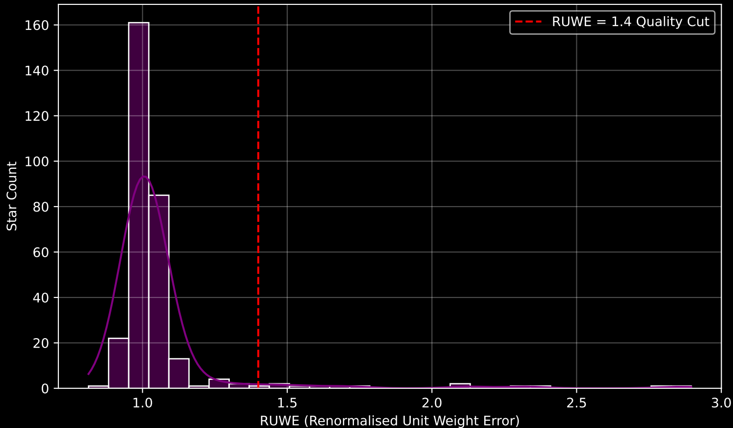
GAPOGEE DR17 Field [345+14] RUWE Distribution (n= 302)
