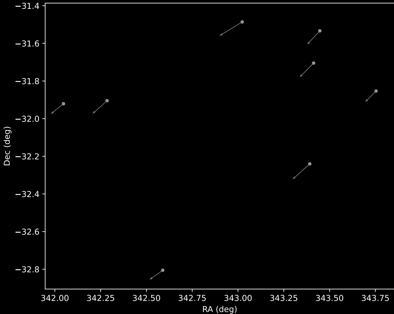
APOGEE DR17 Cluster 14 Proper Motion Vectors (n=8)
