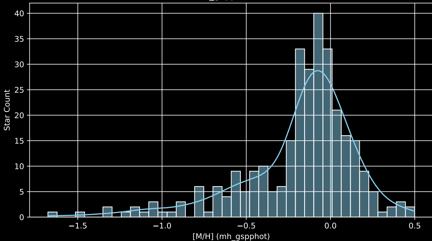
APOGEE DR17 Field: [345+14 [M/H] (mh_gspphot) (n= 301)
