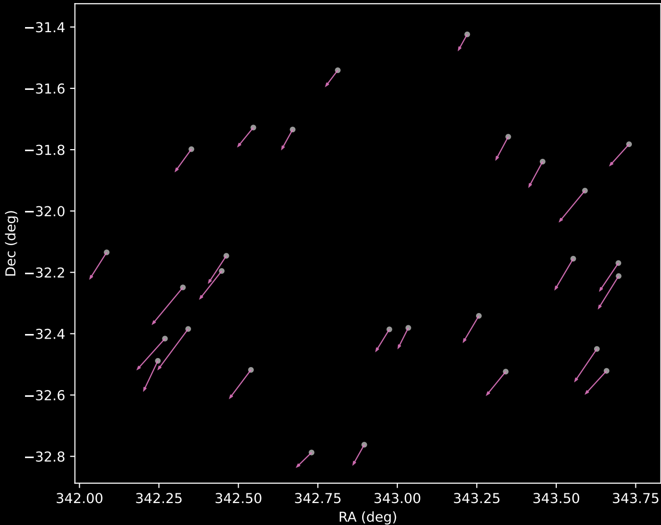
APOGEE DR17 Cluster 12 Proper Motion Vectors (n=28)
