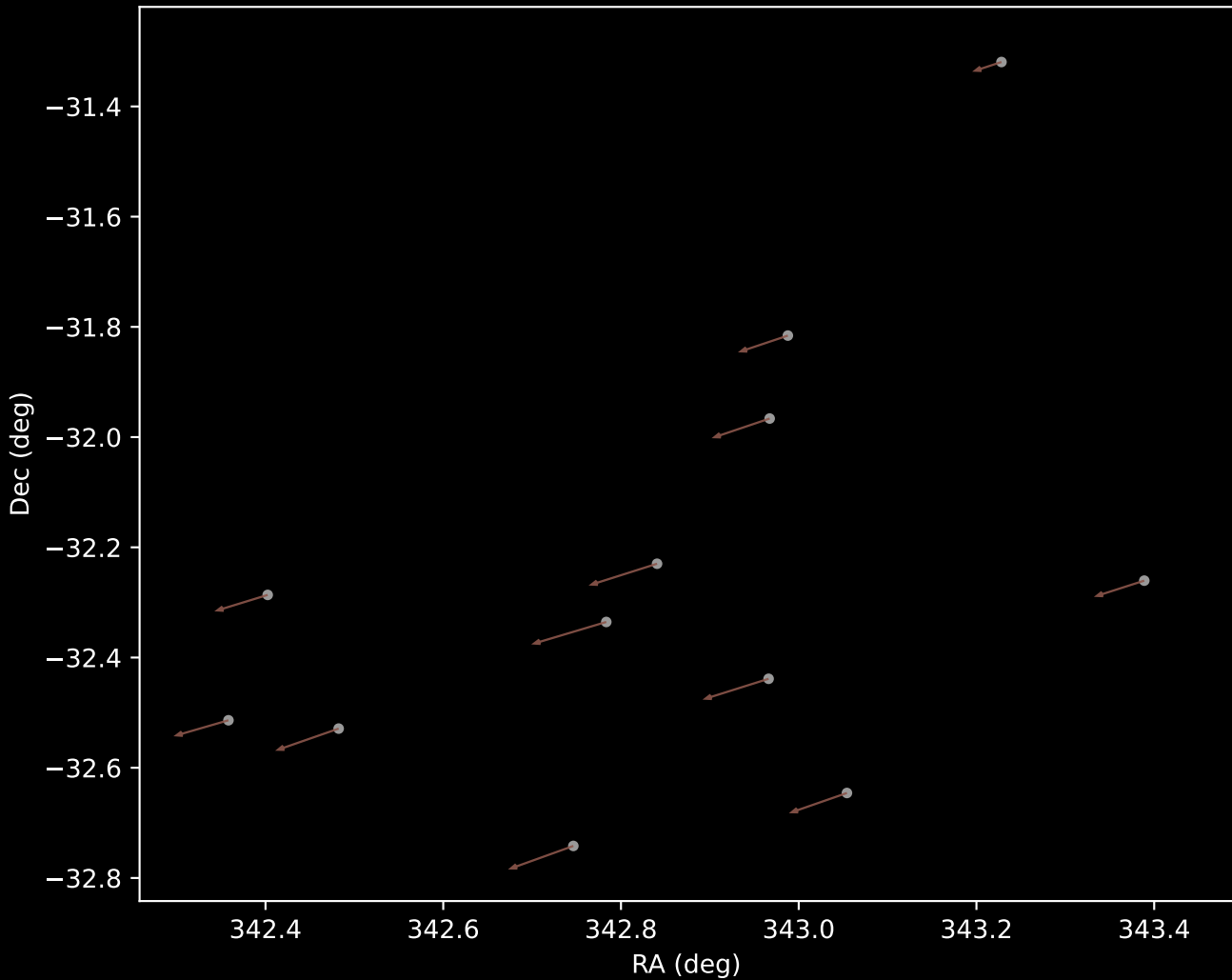
APOGEE DR17 Cluster 10 Proper Motion Vectors (n=12)
