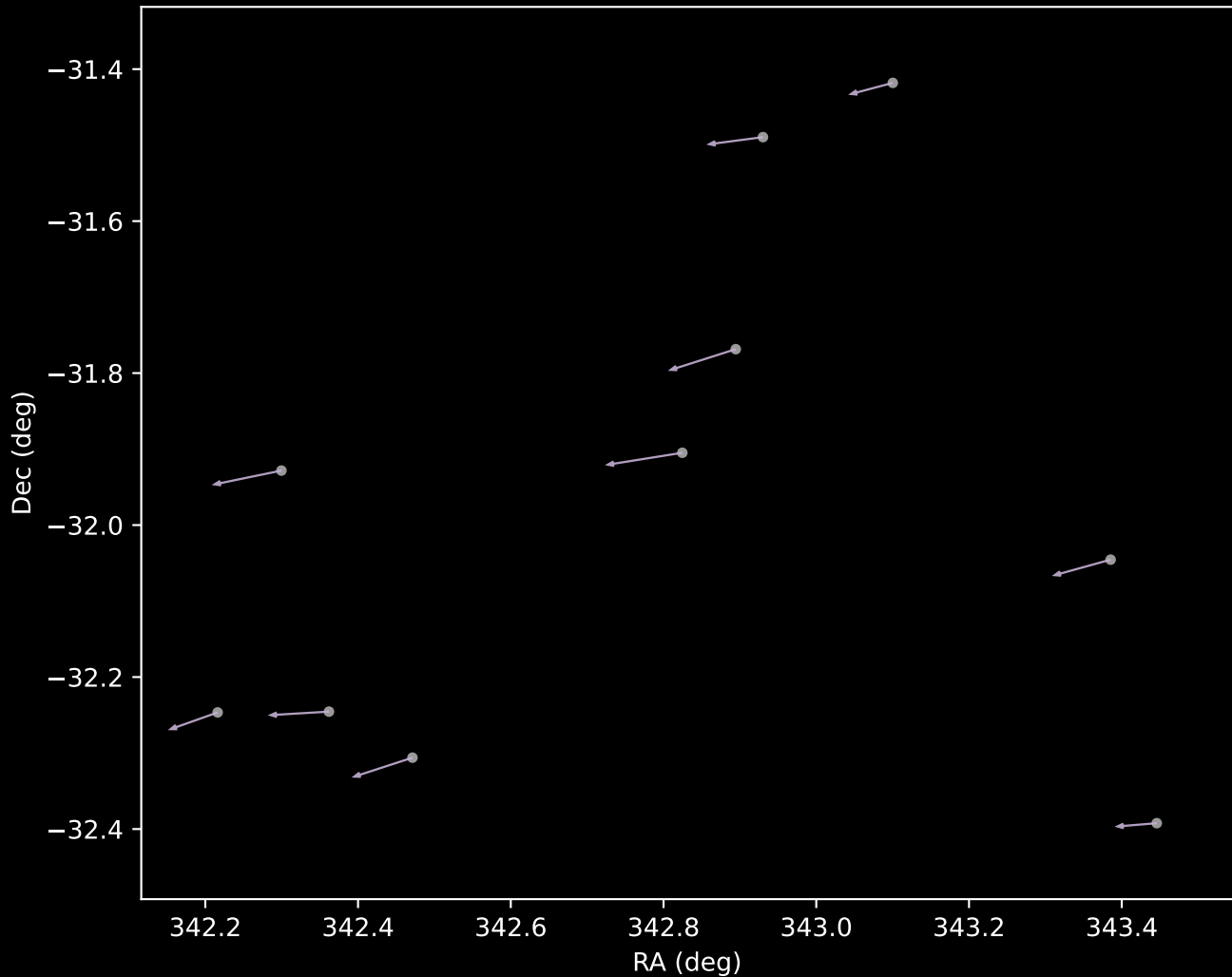
APOGEE DR17 Cluster 9 Proper Motion Vectors (n=10)
